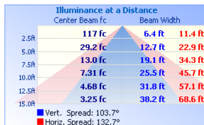
Light Distance: (Illuminance at a Distance)
