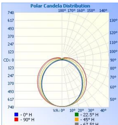
X° Beam Angle: (Polar Candela Dist. )
